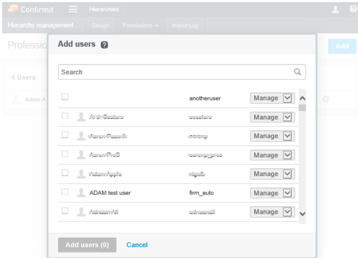
Figure 13 The Add users overlay
