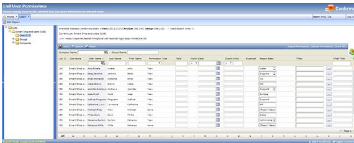
Figure 68 End User Permissions with “Node assignments from Hierarchy Management” enabled
